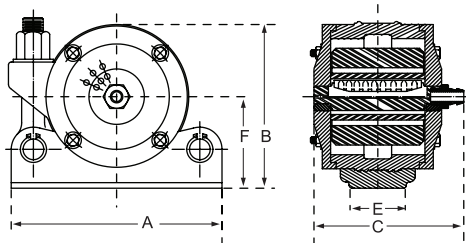
CCR-4400 (shown with bracket 29734)
