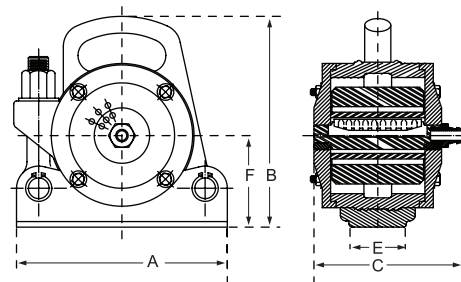
CCR-5500, 6500 (shown with bracket 28732)
