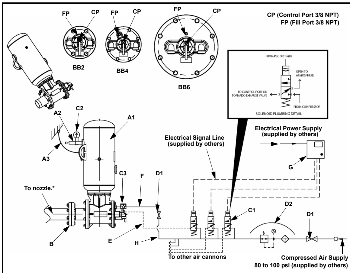
Plumbing Detail for Normally-Closed Solenoid Valve
