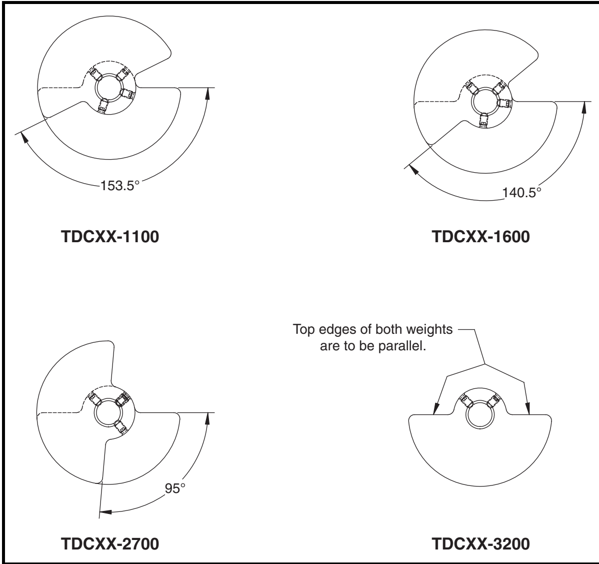
Figure 7. Eccentric Weight Settings
