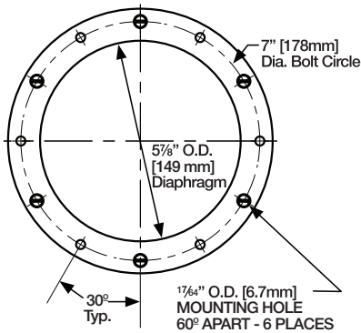
DIAPHRAGM END VIEW
