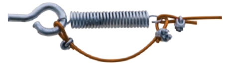
Spring Tensioning Kit with cable safety link. (included with every RSB unit)
