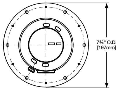
TOP COVER END VIEW
