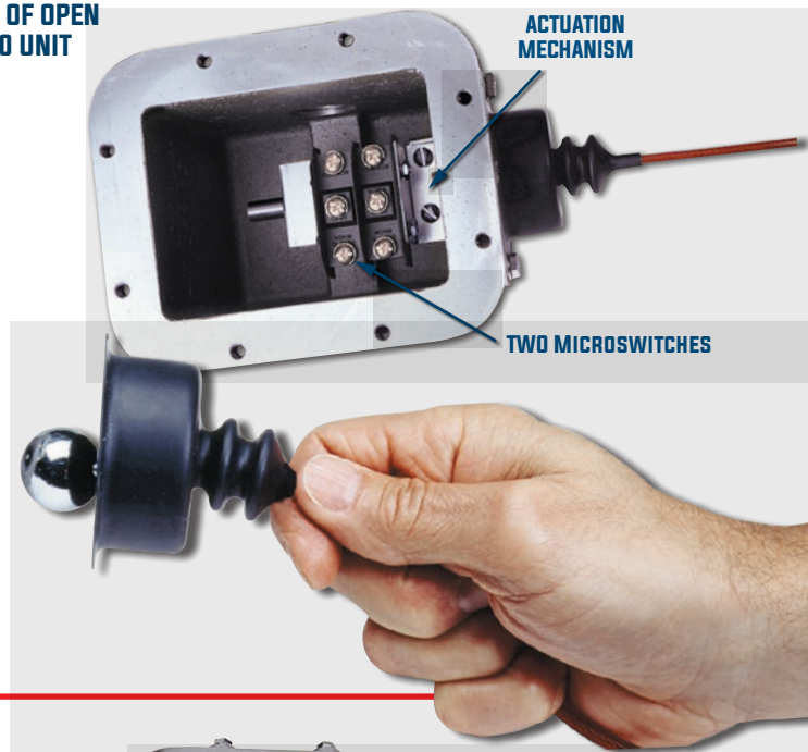
DB-100 unit shown with cable mounting bracket (included).
